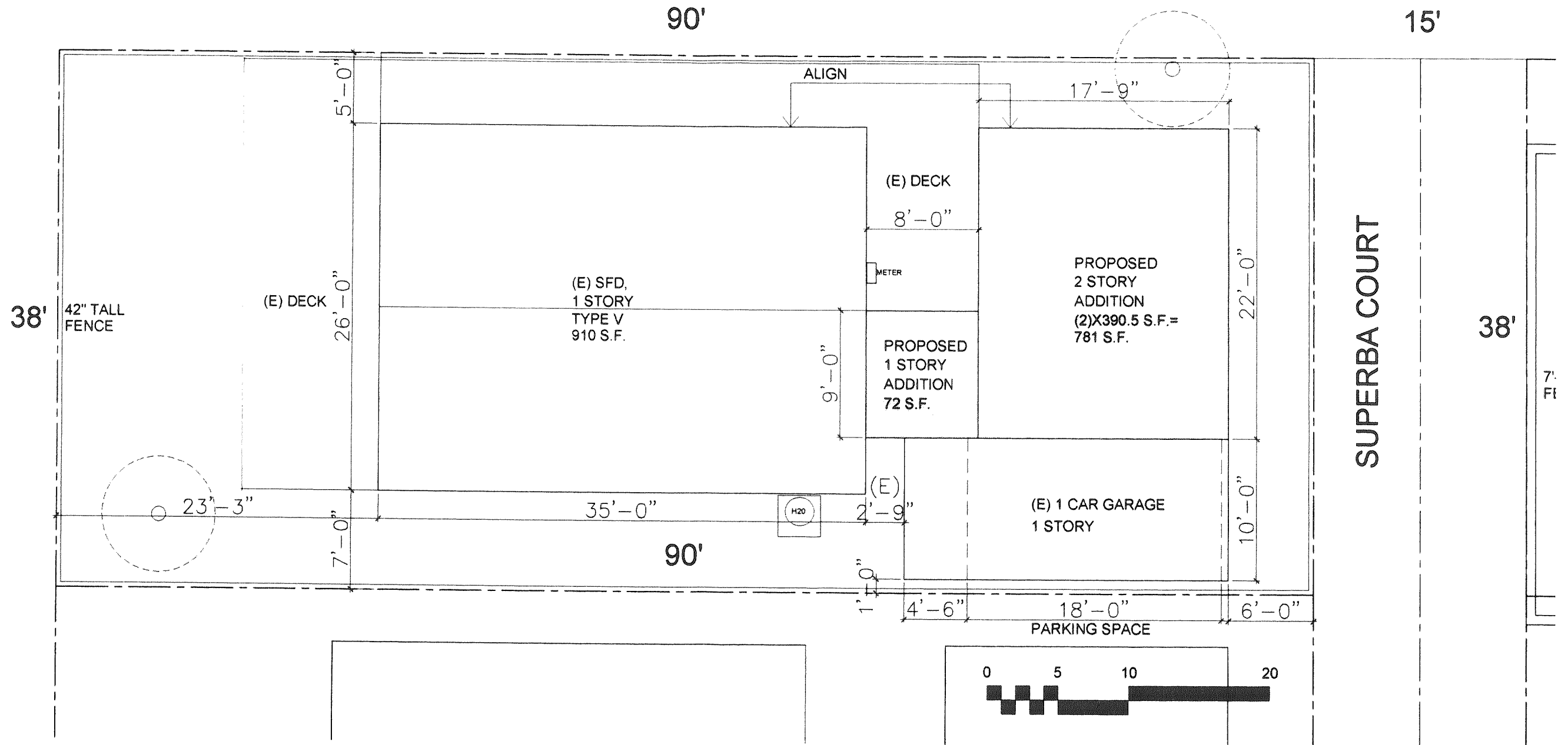
Proposed Site Plan 1/8"=1'-0"
