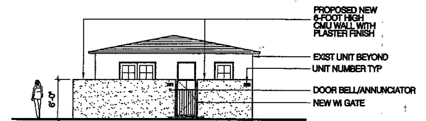
SOUTH ELEVATION
