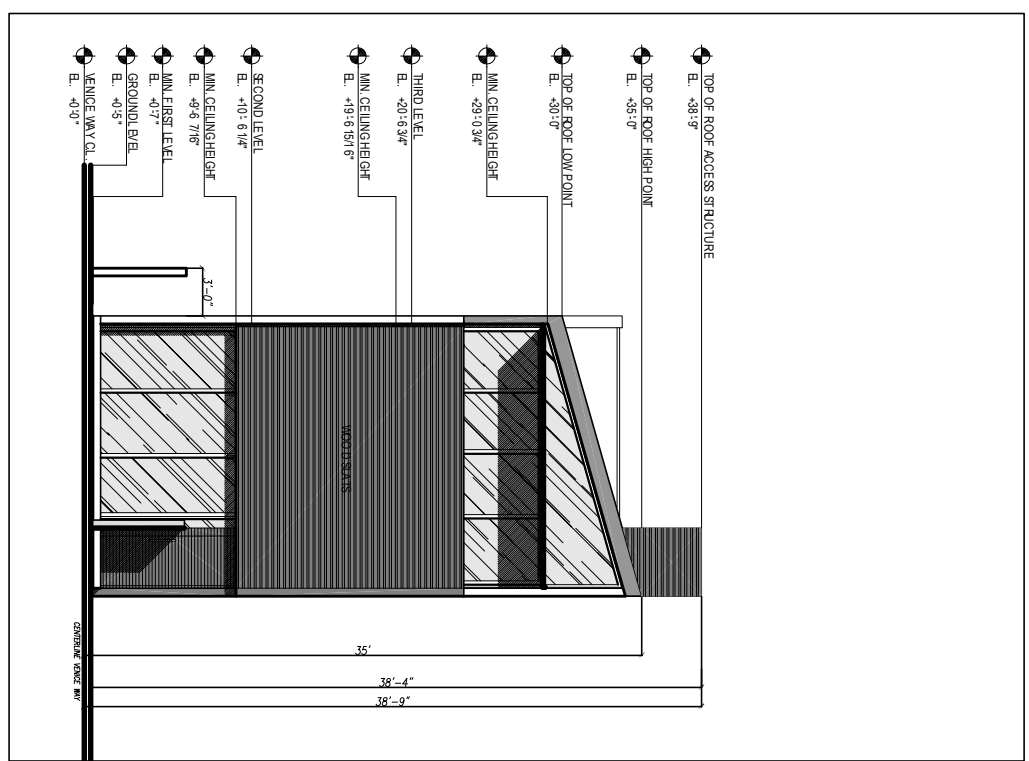
SOUTH ELEVATION
