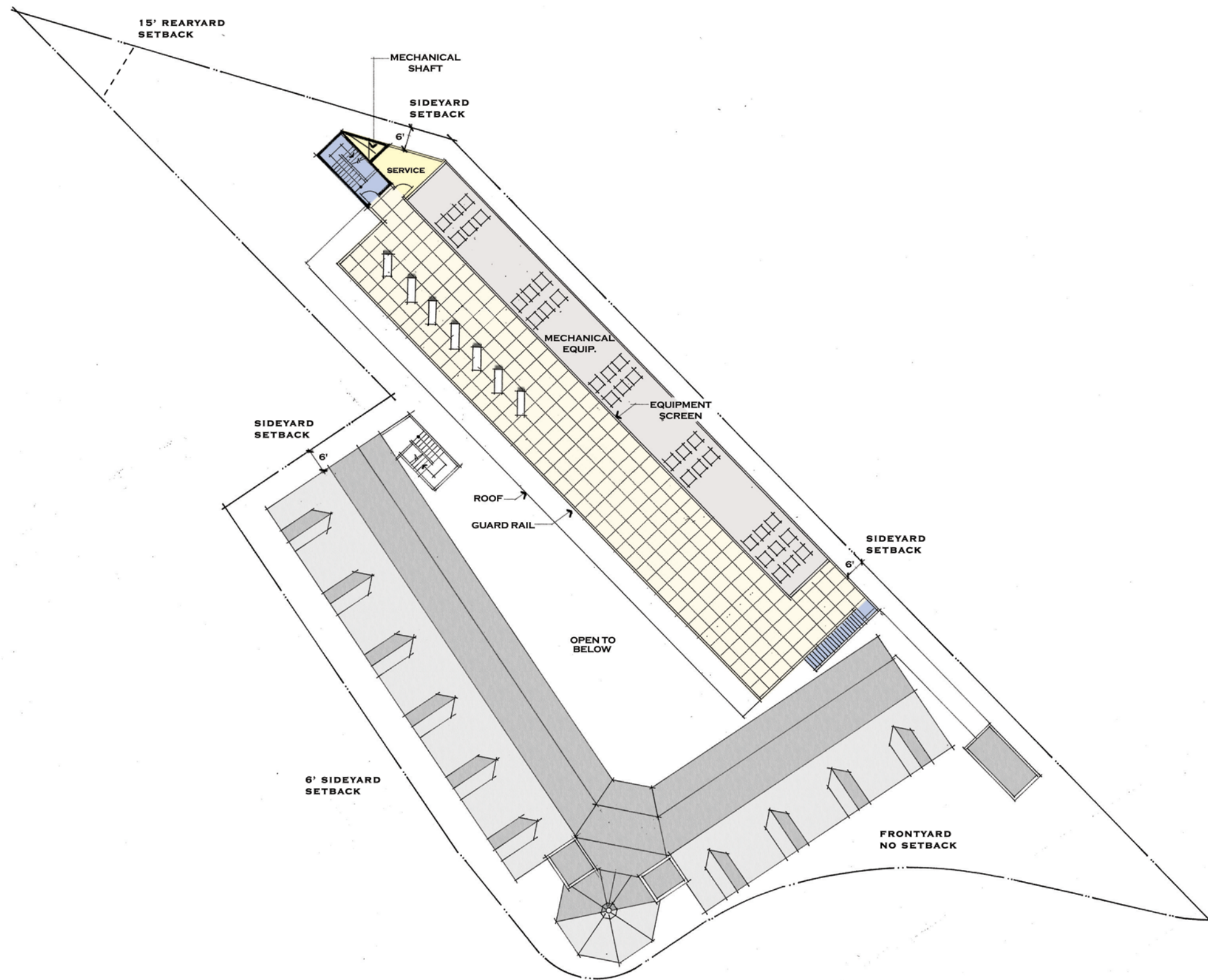
Roof Plan Scale 1/32" = 1'-0"
