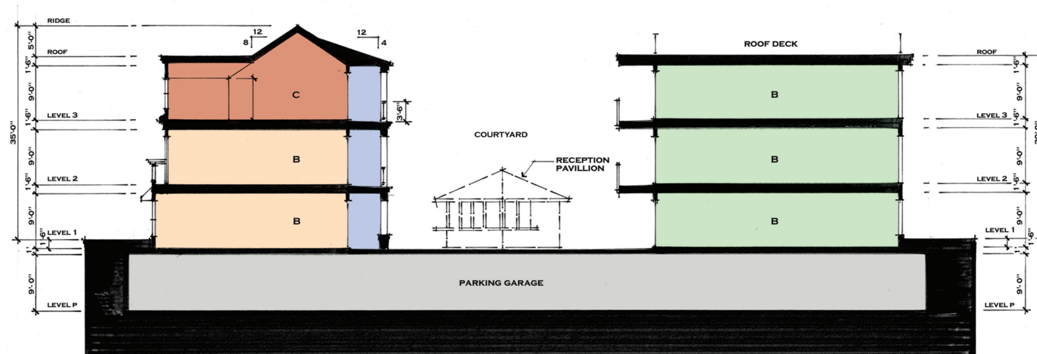
Building Section Scale 1/32" = 1'-0"
