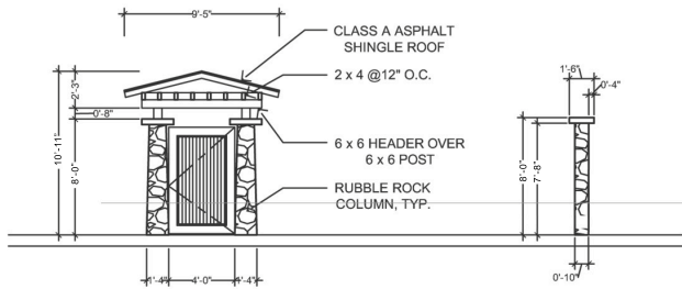
ENTRY STRUCTURE
