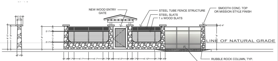
ELEVATION OF FENCE
