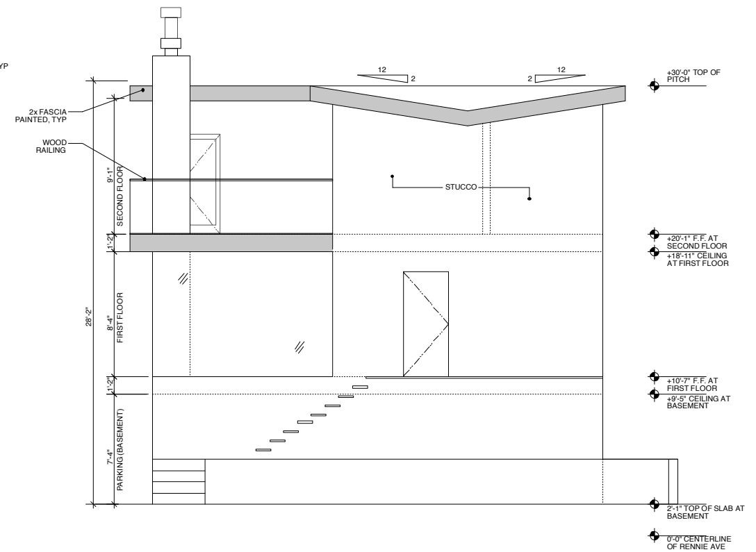
UNIT 3 SOUTHEAST ELEVATION 1 (FRONT FACING UNIT 2)
