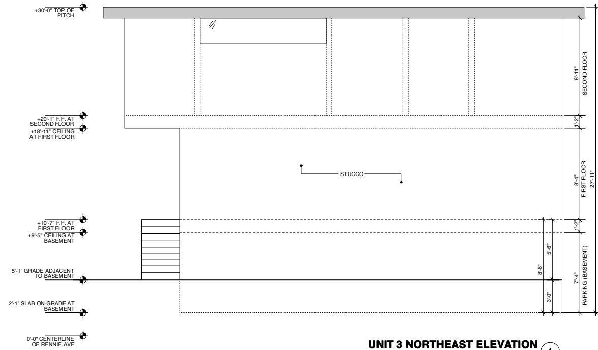
UNIT 3 NORTHEAST ELEVATION 4 (SIDE FACING 5' SETBACK AND NEIGHBORING PROPERTY)
