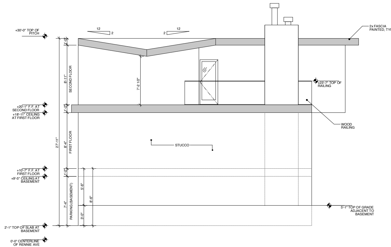
UNIT 3 SOUTHWEST ELEVATION 2 (SIDE FACING EASEMENT WALKWAY)
