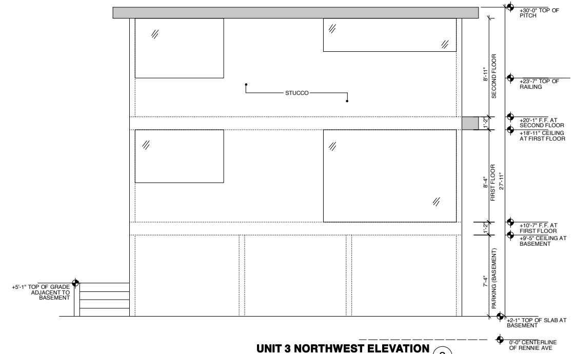
UNIT 3 NORTHWEST ELEVATION 3 (REAR FACING ALLEY)
