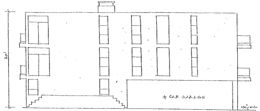
WEST ELEVATION
