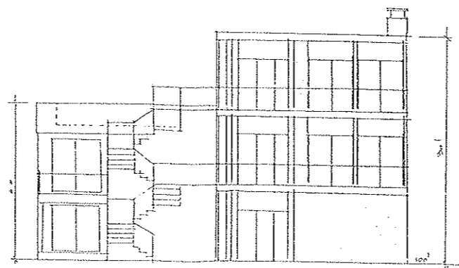
NORTH ELEVATION
